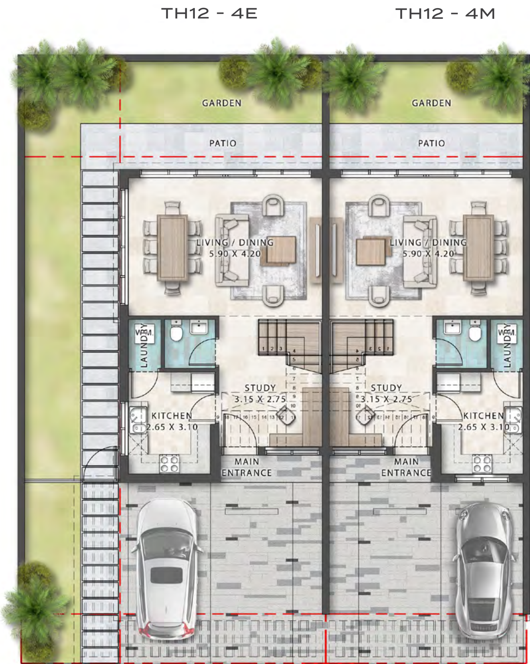
GROUND FLOOR
