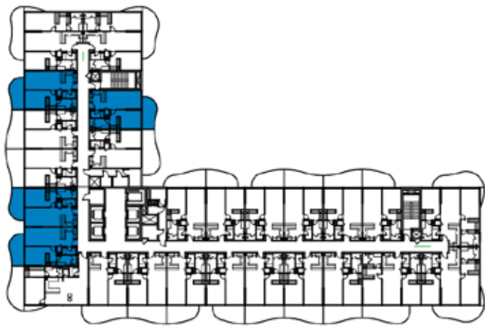
LEVELS: 2, 5, 8 & 11
