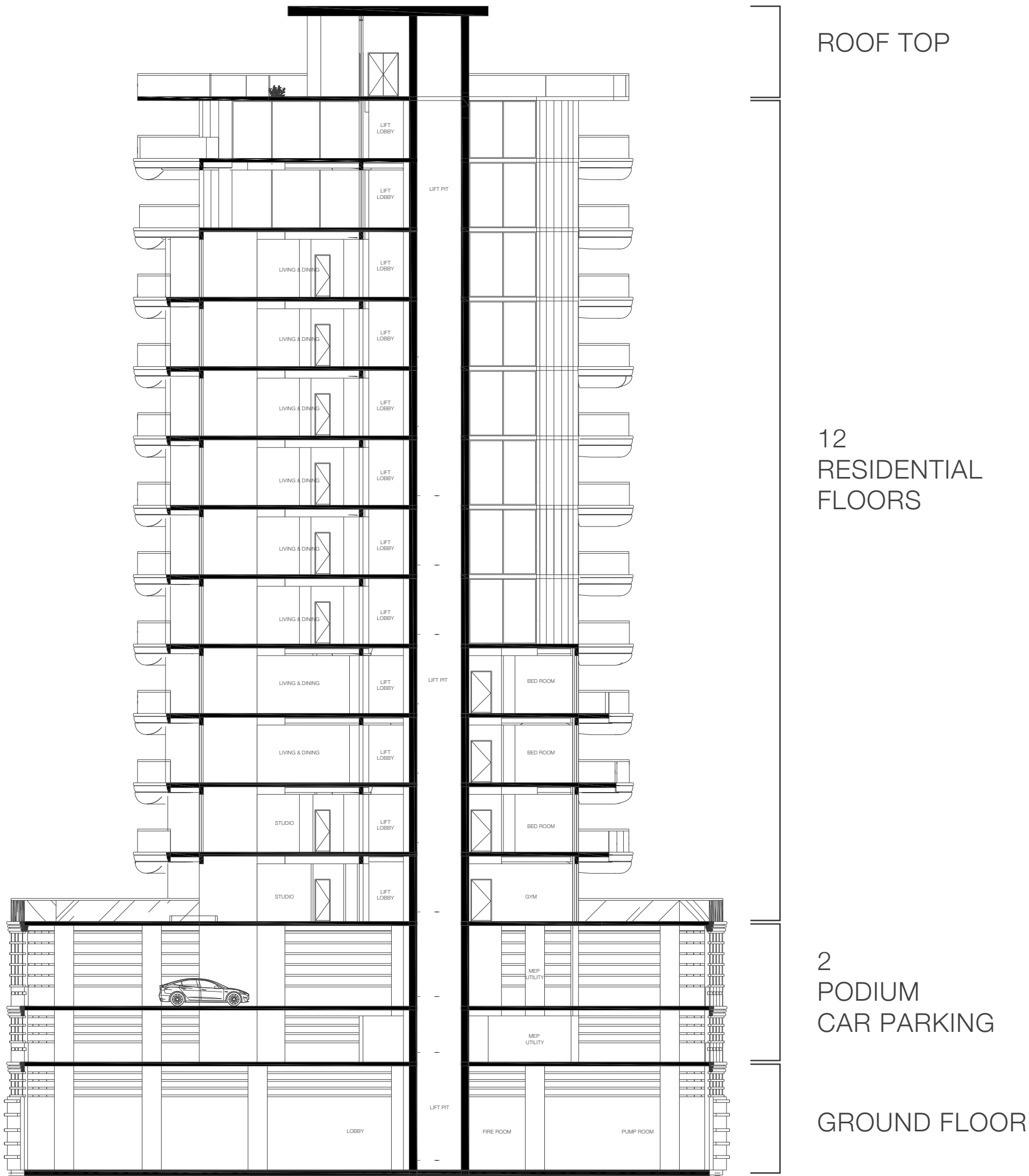
G + 2 PODIUM CAR PARKING + 12 RESIDENTIAL FLOORS
