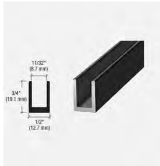
Vertical Aluminum U- Channel: CRL SDCD516MBL Matte Black 5/16" Single Aluminum U-Channel
